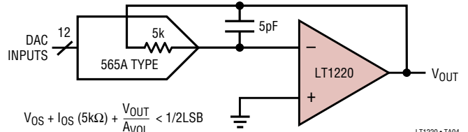
DAC Current-to-Voltage Converter
