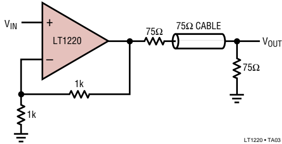
Cable Driver
