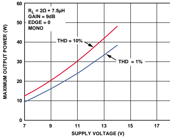
Figure 22. Maximum Output Power vs. Supply Voltage; R_L = 2\Omega ; Mono Mode; THD + N = 1%, THD + N = 10%
