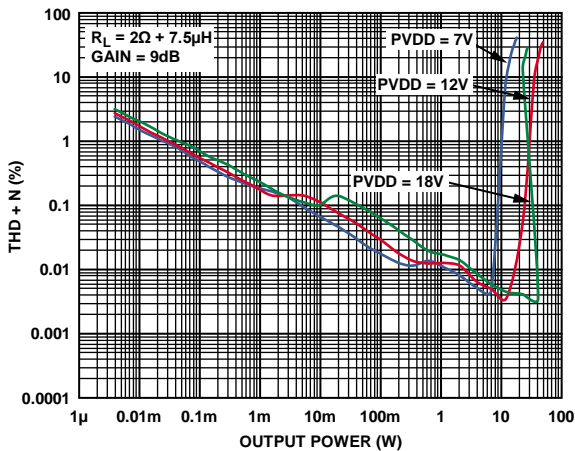
Figure 5. THD + N vs. Output Power into 2 Ω; Mono Mode; Gain = 9 dB; PVDD = 7V, PVDD = 12V, PVDD = 18V
