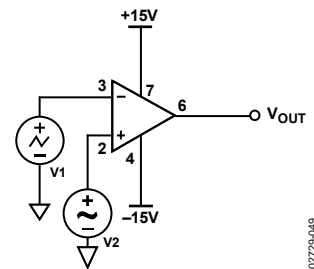
Figure 54. Pulse-Width Modulator
