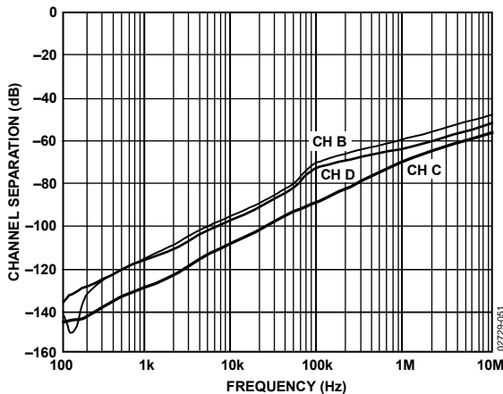
Figure 57. Channel Separation
