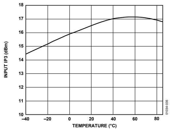
Figure 35. Input IP3 Performance Over Temperature; f_{IN} = 2400 MHz, f_{OUT} = 425 MHz
