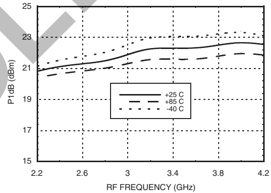
Input P1dB vs. Temperature @ LO = +17 dBm
