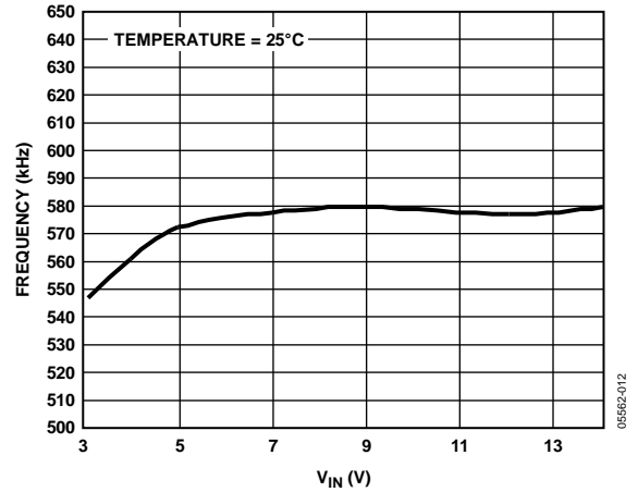
Figure 11. Oscillator Frequency vs. Input Voltage
