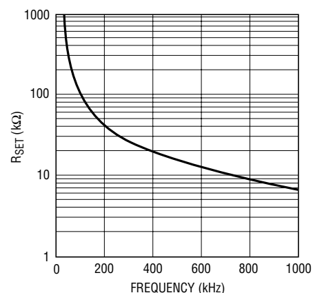
Figure 6. Timing Resistor ( R_{SET} ) Value
