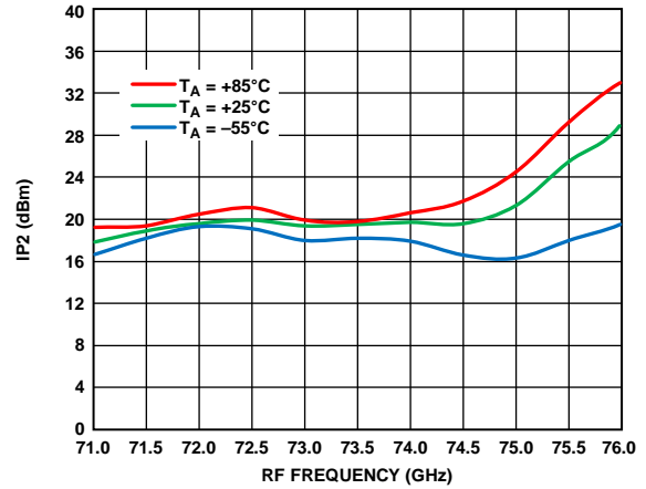
Figure 30. Input IP2 vs. RF Frequency at Various Temperatures, R_{FIN} = -20 dBm, LO = 2 dBm, IF = 1000 MHz, V_{DLNA} = 3 V
