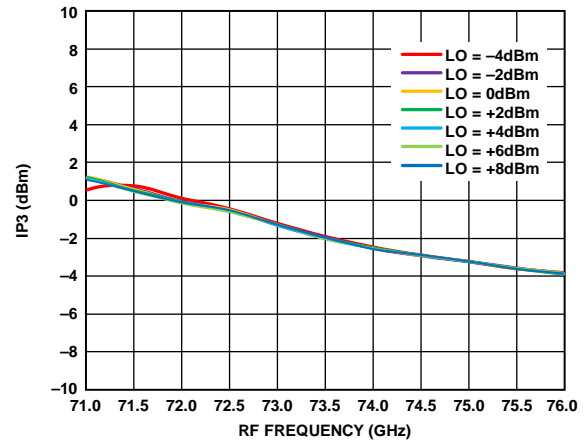
Figure 86. Input IP3 vs. RF Frequency at Various LO Powers, RF_{IN} = -20 dBm, IF = 2000 MHz, V_{DLNA} = 3 V
