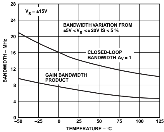
TPC 20. OP15 Bandwidth vs. Temperature
