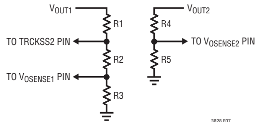
Figure 7. Alternative Setup for Coincident Tracking
