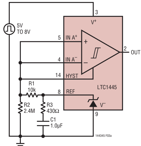
Figure 3a. V^+ Glitching Test Circuit
