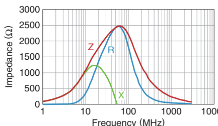
MMZ1608Y600BTD25
