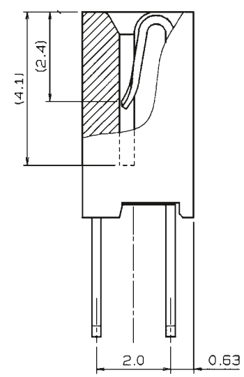
SECT X-X
