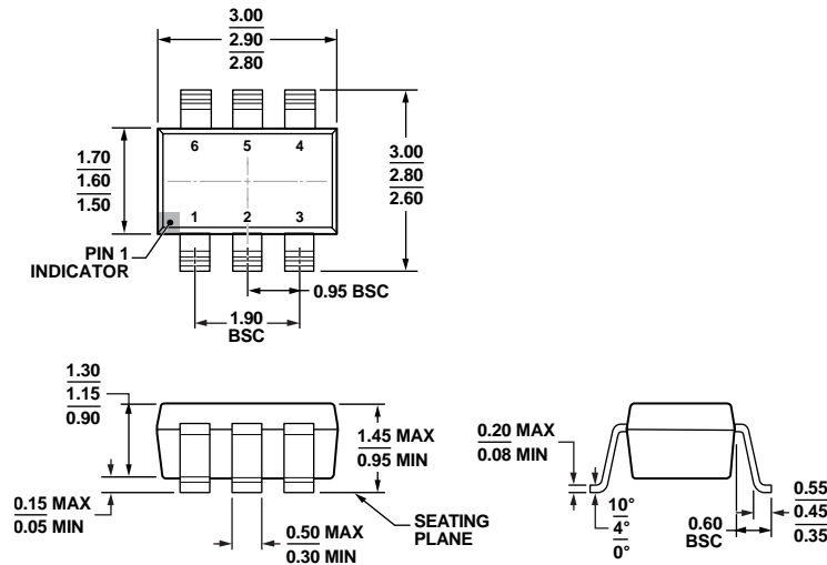
COMPLIANT TO JEDEC STANDARDS MO-178-AB Figure 70. 6-Lead Small Outline Transistor Package [SOT-23] (RJ-6) Dimensions shown in millimeters
