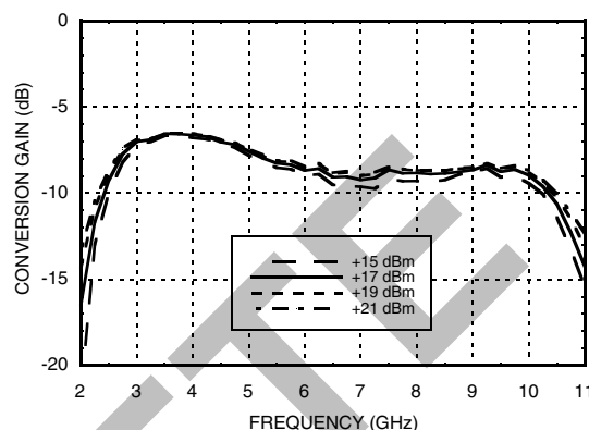
Upconverter Performance Conversion Gain vs. LO Drive, IF Frequency 100 MHz
