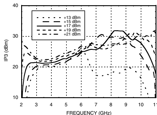
Input IP3 vs. LO Drive*, IF Frequency = 100 MHz
