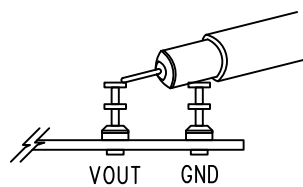
Figure 5. Measuring Output Ripple
