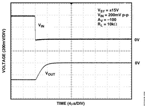
Figure 24. Negative Overdrive Recovery
