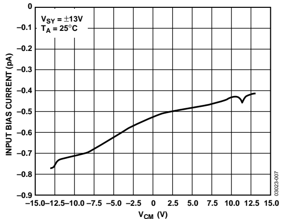
Figure 7. Input Bias Current vs. V_{CM}
