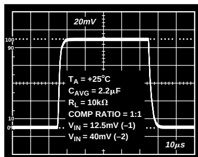
Figure 8. Small Signal Transient Response
