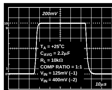
Figure 9. Large Signal Transient Response
