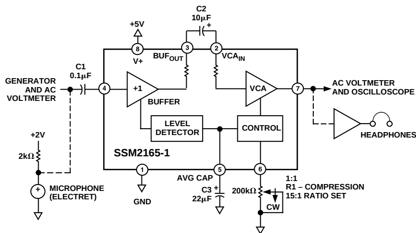
Figure 16. Electret Microphone Preamp Example
