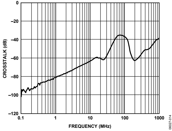
Figure 19. Crosstalk
