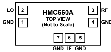
Figure 2. Pad Configuration
