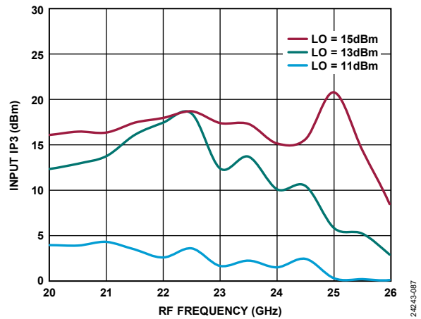
Figure 83. Input IP3 vs. RF Frequency at Various LO Power Levels, TA = 25°C
