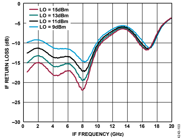
Figure 93. IF Return Loss vs. IF Frequency at Various LO Power Levels, T_A = 25^\circ\text{C} , LO = 15 GHz
