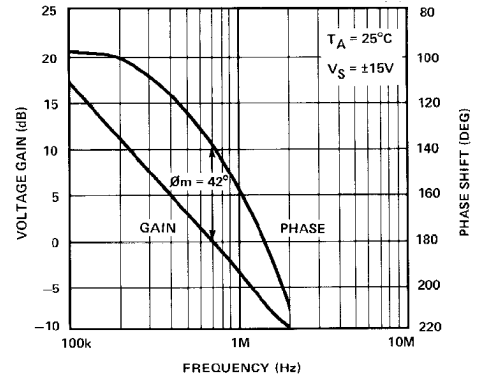
GAIN AND PHASE SHIFT vs FREQUENCY
