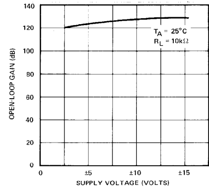
OPEN-LOOP GAIN vs SUPPLY VOLTAGE
