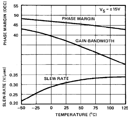
PHASE MARGIN, GAIN-BANDWIDTH, AND SLEW RATE vs TEMPERATURE
