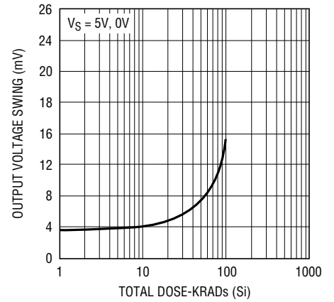
Output Voltage Swing Low, No Load
