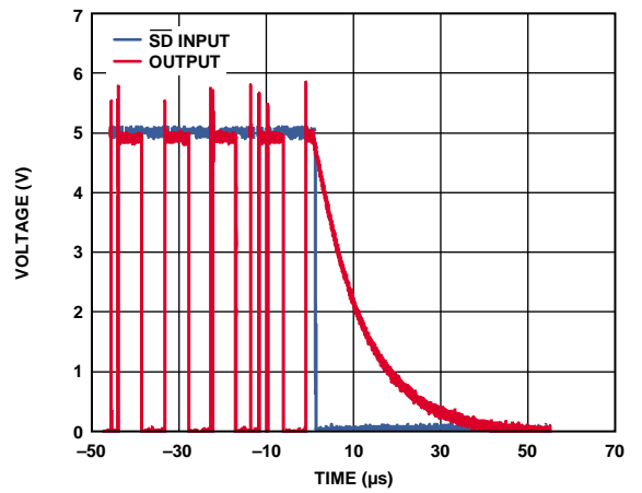
Figure 32. Turn-Off Response
