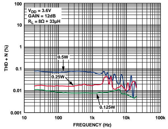
Figure 13. THD + N vs. Frequency, V_{DD} = 3.6V , R_L = 8\Omega , Gain = 12 dB
