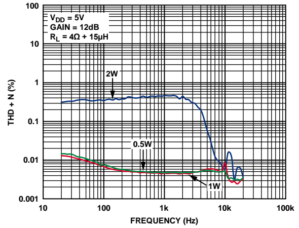
Figure 12. THD + N vs. Frequency, V_{DD} = 5V , R_L = 4\Omega , Gain = 12 dB
