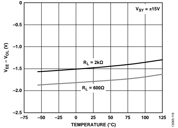
Figure 19. Output Saturation Voltage ( V_{EE} - V_{OL} ) vs. Temperature, V_{SY} = \pm 15 V
