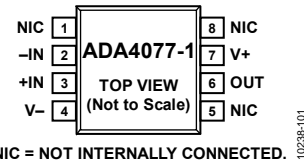
Figure 1. ADA4077-1, 8-Lead SOIC and 8-Lead MSOP
