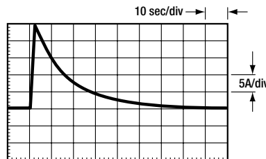
Fig. 4b. Lightning strike pulse, example #4.
