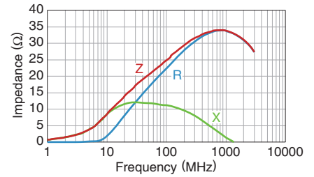
MPZ1608S300ATDH5
