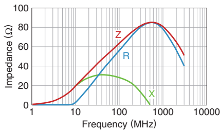
MPZ1608S600ATDH5
