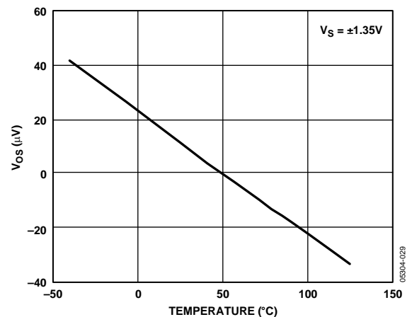
Figure 34. Input Offset Voltage vs. Temperature
