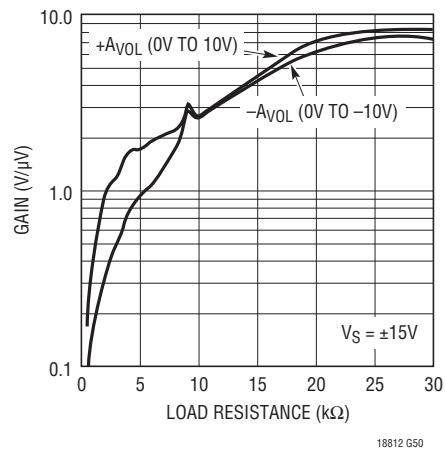
Gain vs Load Resistance
