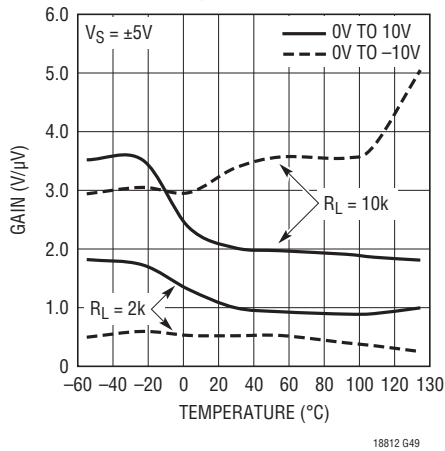
Gain vs Temperature
