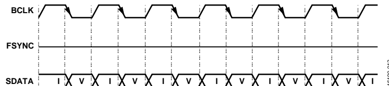
Figure 69. SDATA Output in PDM Mode
