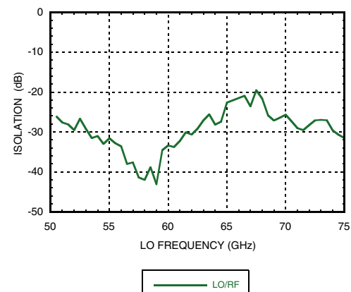
LO/RF isolation
