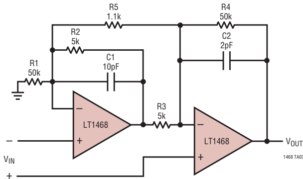
Instrumentation Amplifier
