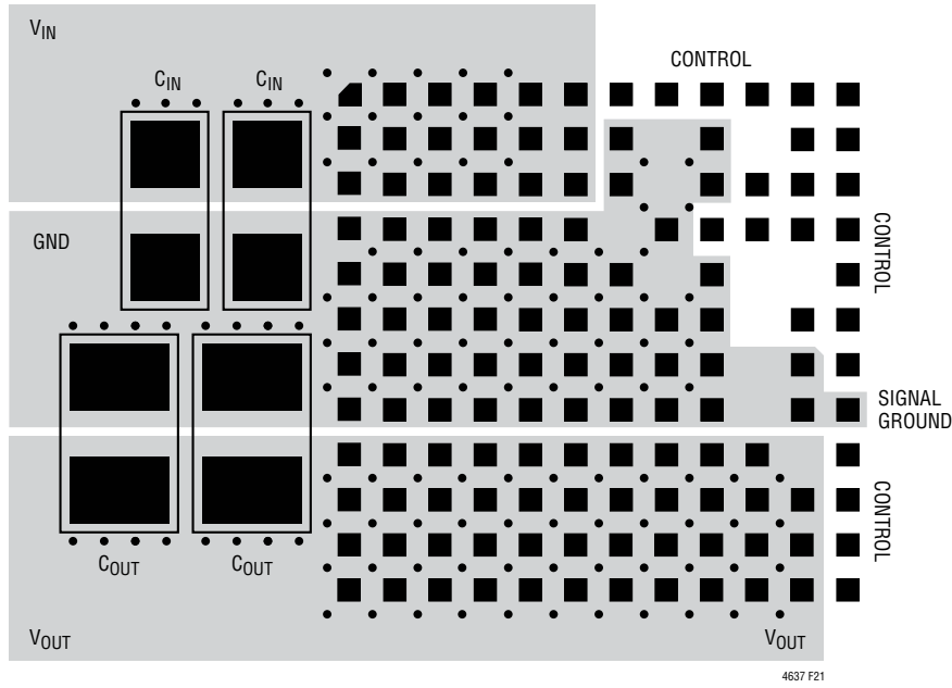
Figure 21. Recommended PCB Layout (LGA Shown, for BGA Use Circle Pads)
