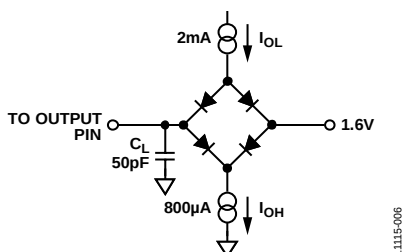
Figure 6. Load Circuit for Timing Specifications
