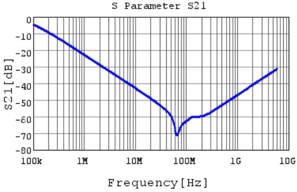
NFM18PC104R1C3 S21 DCOV,25degC, Feedthrough
