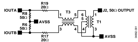
Figure 93. IF Signal Output Circuit
