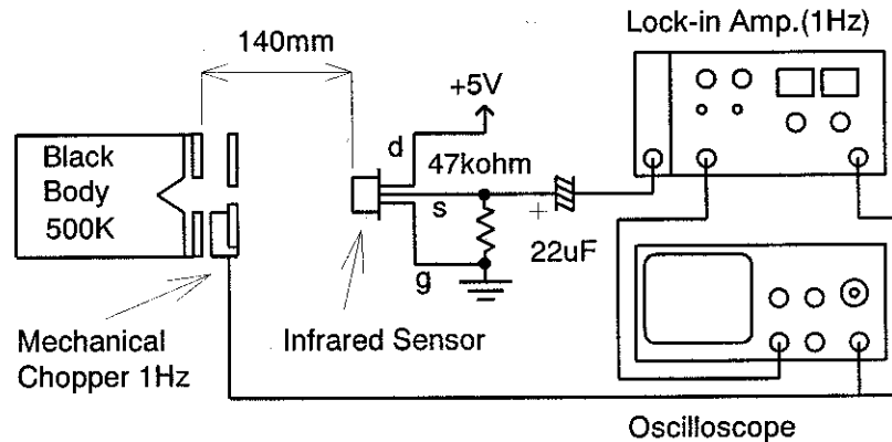
Figure 1. Test system of responsivity
