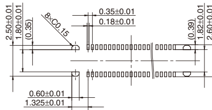
Recommended metal mask pattern Metal mask thickness: When 100μm (Terminal opening ratio: 70%) (Metal-part opening ratio: 46%)
