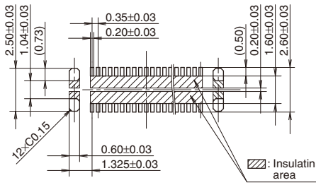
Recommended metal mask pattern Metal mask thickness: When 100μm (Terminal opening ratio: 70%) (Metal-part opening ratio: 46%)
