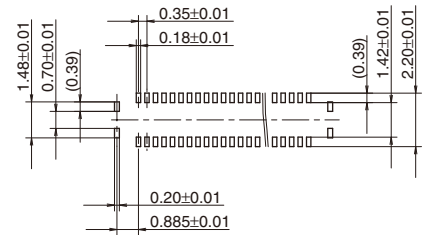
Recommended metal mask pattern Metal mask thickness: When 100μm (Signal terminal opening ratio: 70%) (Power terminal opening ratio: 77%)
