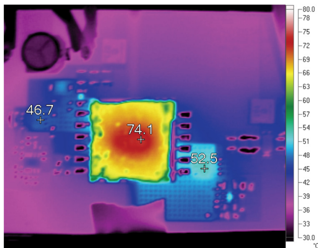
Figure 7. Thermal Picture, 48V IN and 5A OUT ( T_A = 25^\circ C , Air Flow 200LFM) Synchronous MOSFET, 52.5°C; Primary MOSFET, 46.7°C; Transformer, 74.1°C
