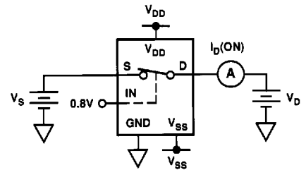
TEST CIRCUIT 3 I_D (ON)
