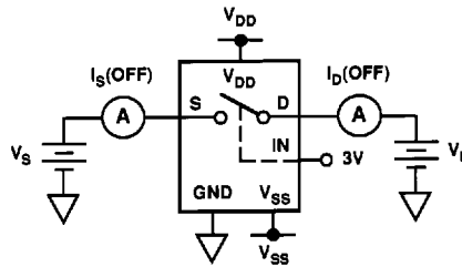
TEST CIRCUIT 2 I_S (OFF), I_D (OFF)
