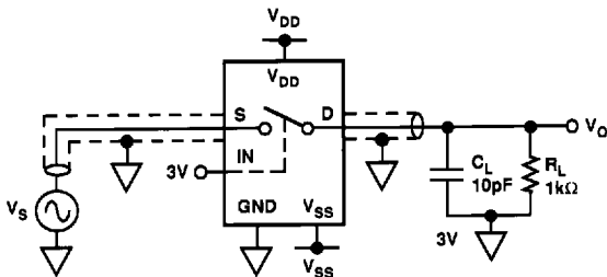
TEST CIRCUIT 5 OFF ISOLATION
