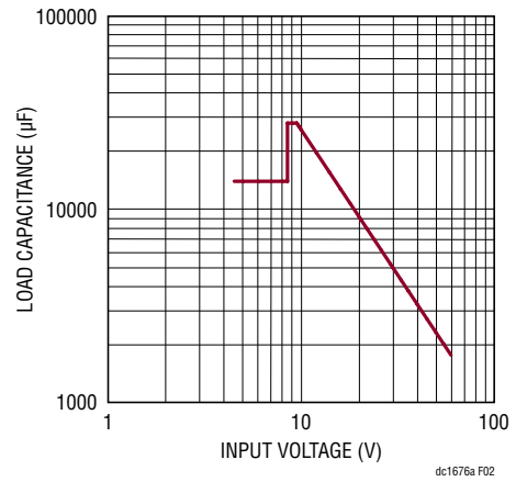
Figure 2. Maximum Permissible Load Capacitance at Start-Up
