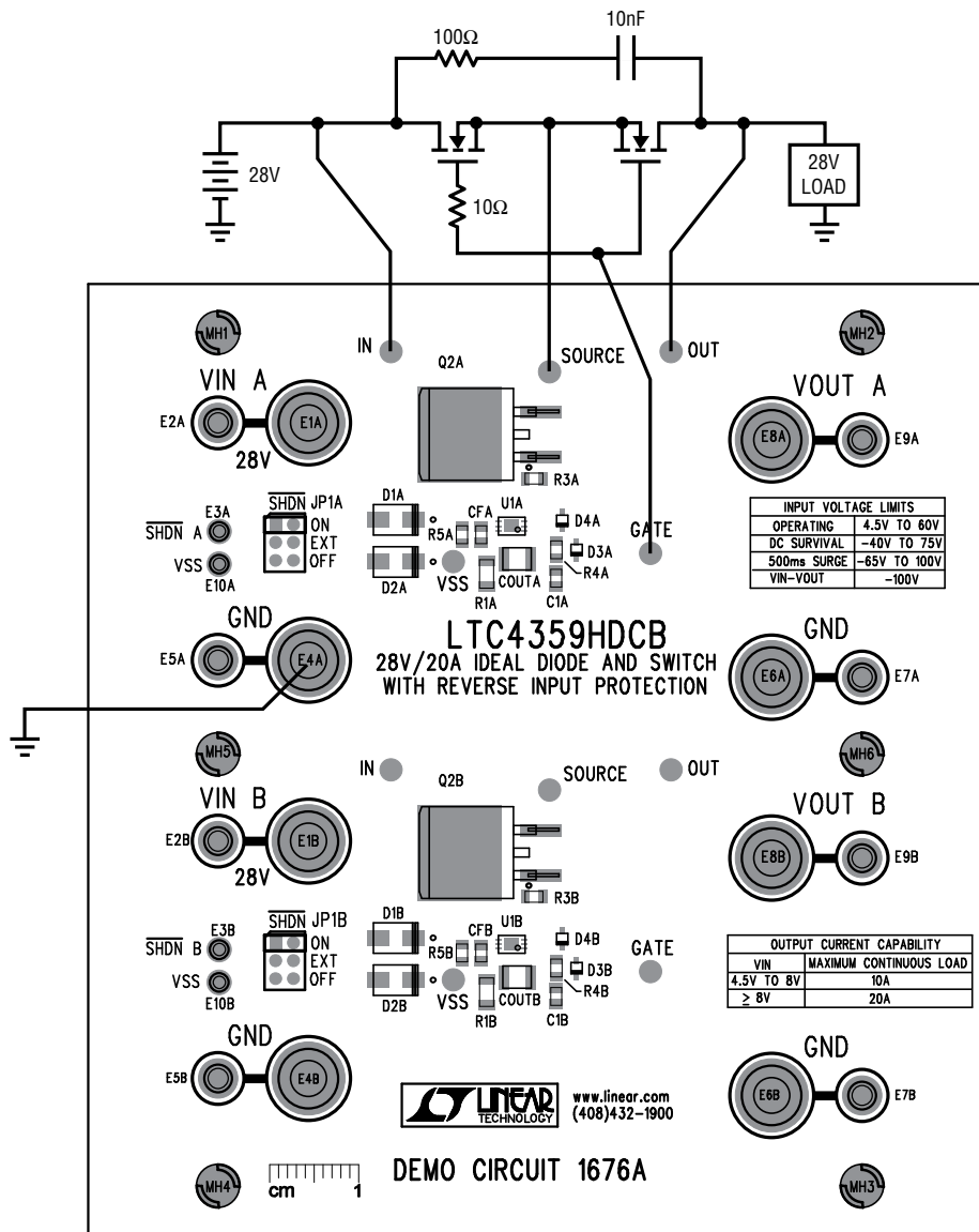
Figure 4. Driving an Off-Board Power Stage. Remove Q1, Q2, RSNUB and CSNUB (See Schematic Diagram)
