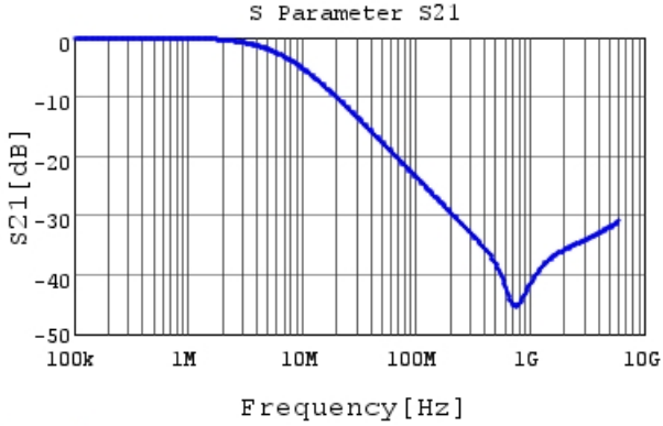
NFM21CC102R1H3 S21 DCOV,25degC, Feedthrough
