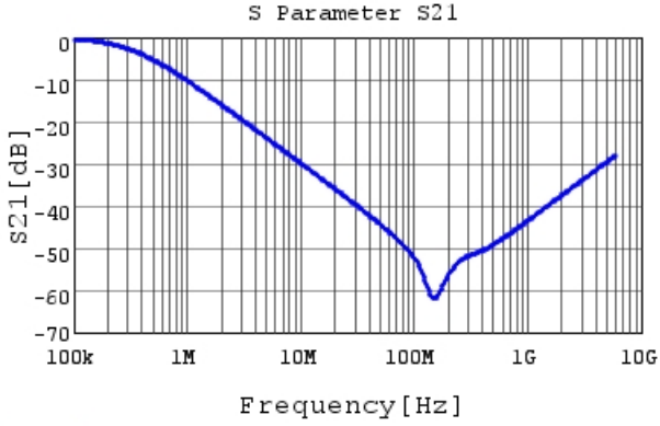
NFM3DPC223R1H3 S21 DCOV,25degC, Feedthrough
