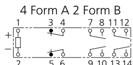
Schematic ( BOTTOM VIEW )
