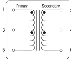
Pin Connections 76253/XXEN (Top View)
