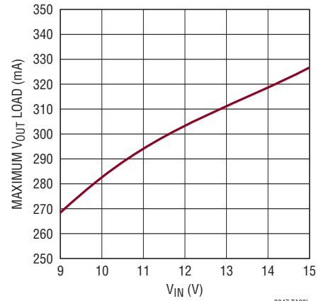
Maximum Load vs V_{IN}
