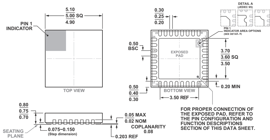
Figure 39. 32-Lead Lead Frame Chip Scale Package [LFCSP_SS] 5 mm x 5 mm Body, With Side Solderable Leads (CS-32-2) Dimensions shown in millimeters
