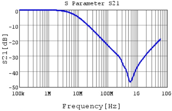
NFM41CC102R2A3 S21 DCOV,25degC, Feedthrough
