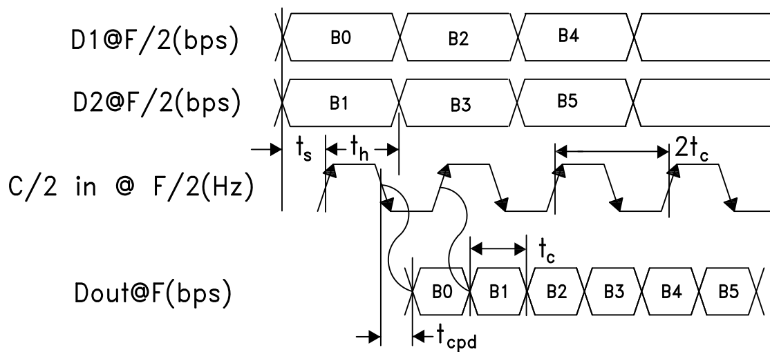
Timing Diagram
